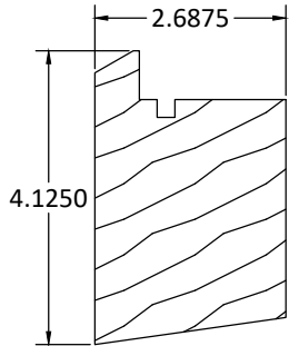
7 LOWER CHECK RAIL
