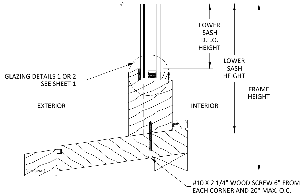
C 4 VERTICAL SECTION SILL
