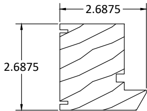
8 GLASS STOP
