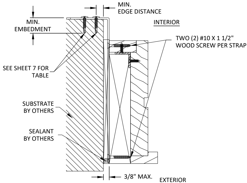
C 6 ANCHOR DETAIL HRS12 STRAP BENT AROUND OPENING - JAMB
