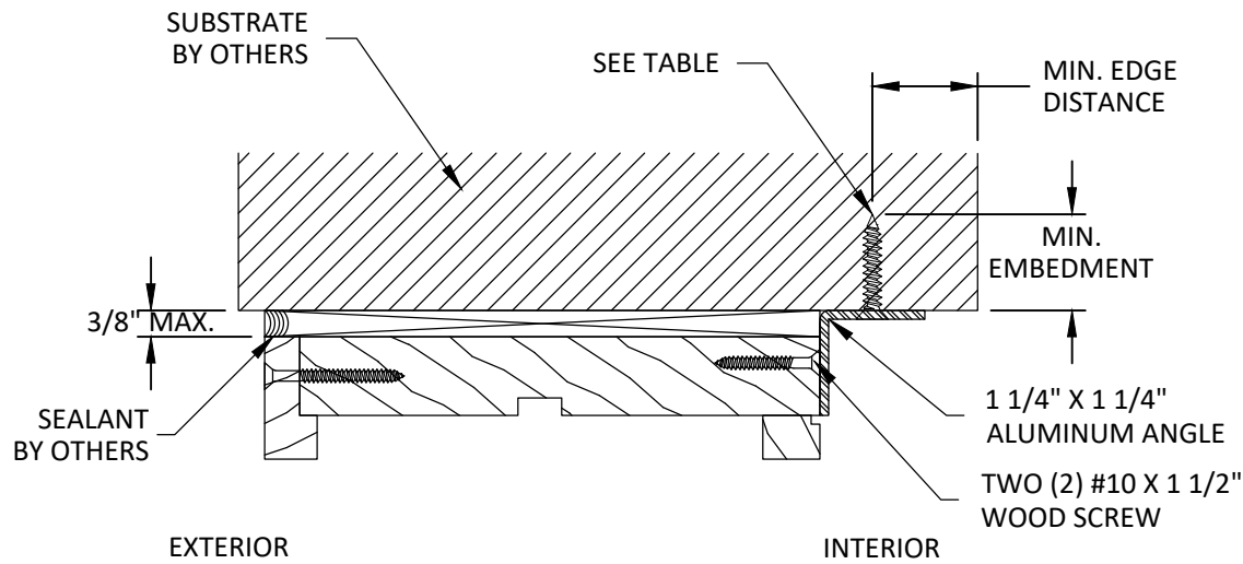
A 7 ANCHOR DETAIL ALUMINUM ANGLE - HEAD
